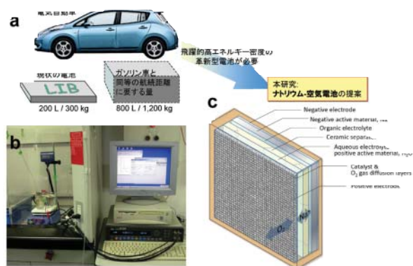
(a) 電気自動車の航続距離の問題 (b) 電池試験 (c) Na-空気電池の概念 (a) Issue in driving range of electronic vehicles. (b) A cell test. (c) Concept of Na-air cell.
